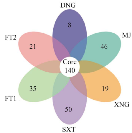
图 5 不同样本组 OTUs 分布 Venn 图 Figure 5 Venn figure of OTUs distribution of different sample groups. DNG, MJ, XNG, SXT, FT1, FT2 represent the name of sampling positions.
